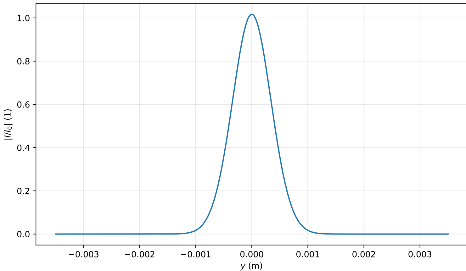
Intensity profile I(x=0, y, z=0.159)/I_0 , P_{in}=0.9P_{cr} , artificial time
